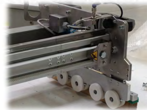
(lengthening device)
